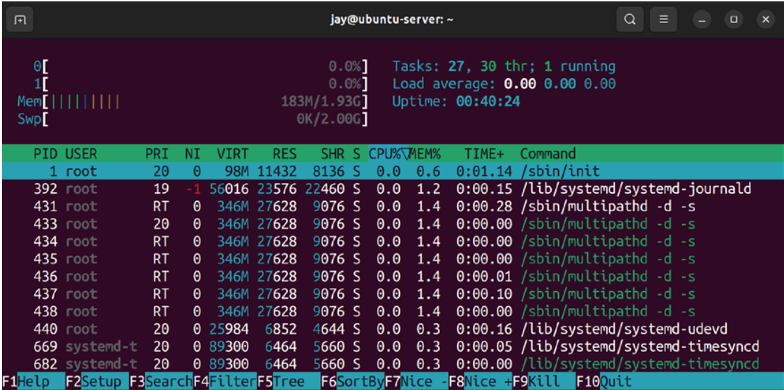
Figure 8.7: Running htop
